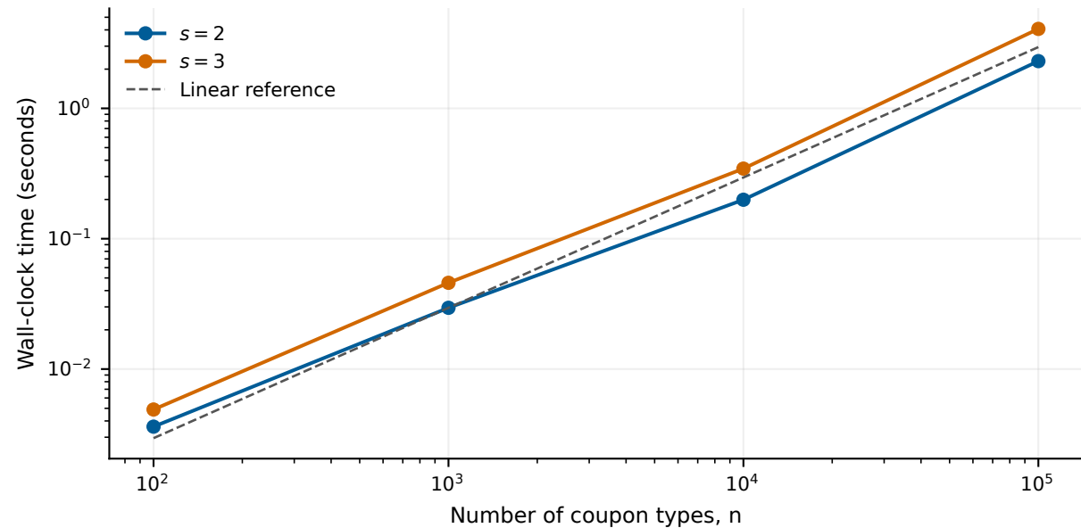
Ungrouped evaluation with 128-bit Arb
