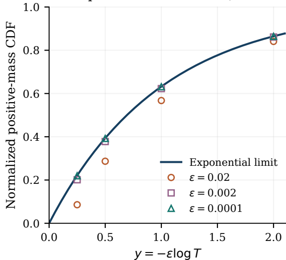
B. Exponential mass scale, b = 1/2
