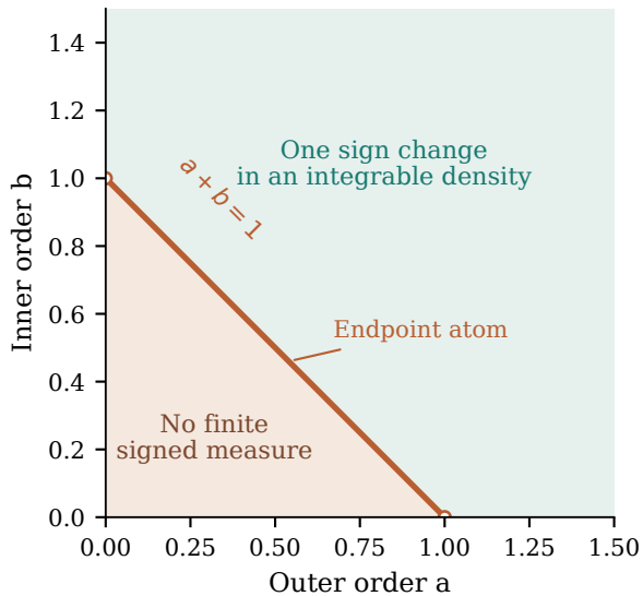
A. Sharp measure threshold
