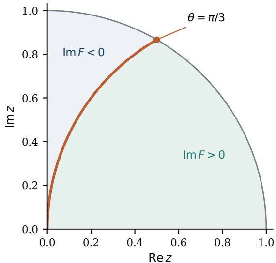
B. Exact zero arc, a = b = 1
