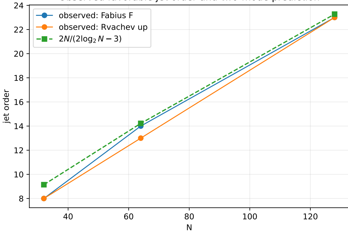
Observed favorable jet order and two-mode prediction
