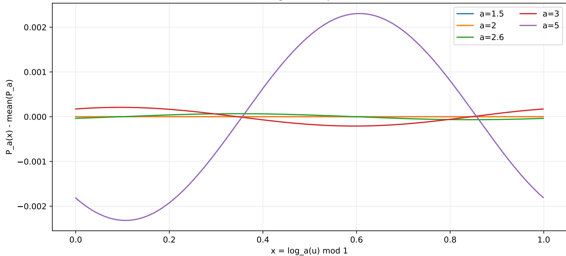
General-base logarithmic periodic correction
