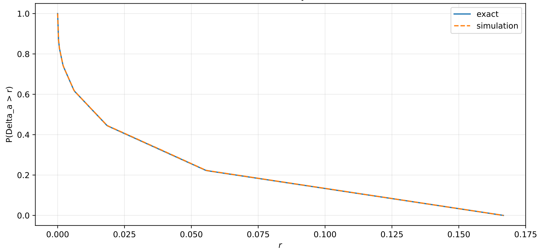
Distance to the nonanalytic set for a=3
