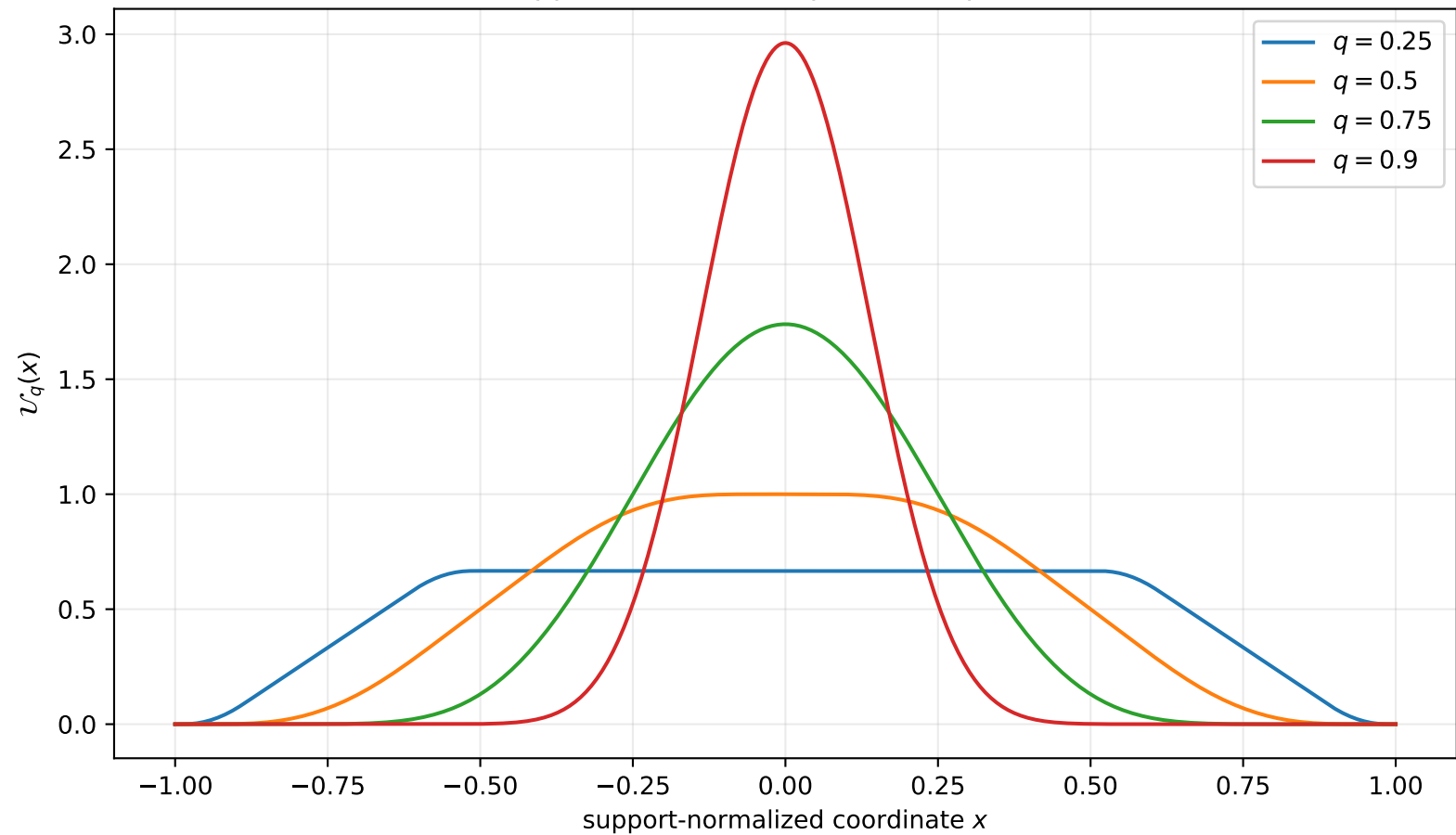
Support-normalized q-Rvachev profiles
