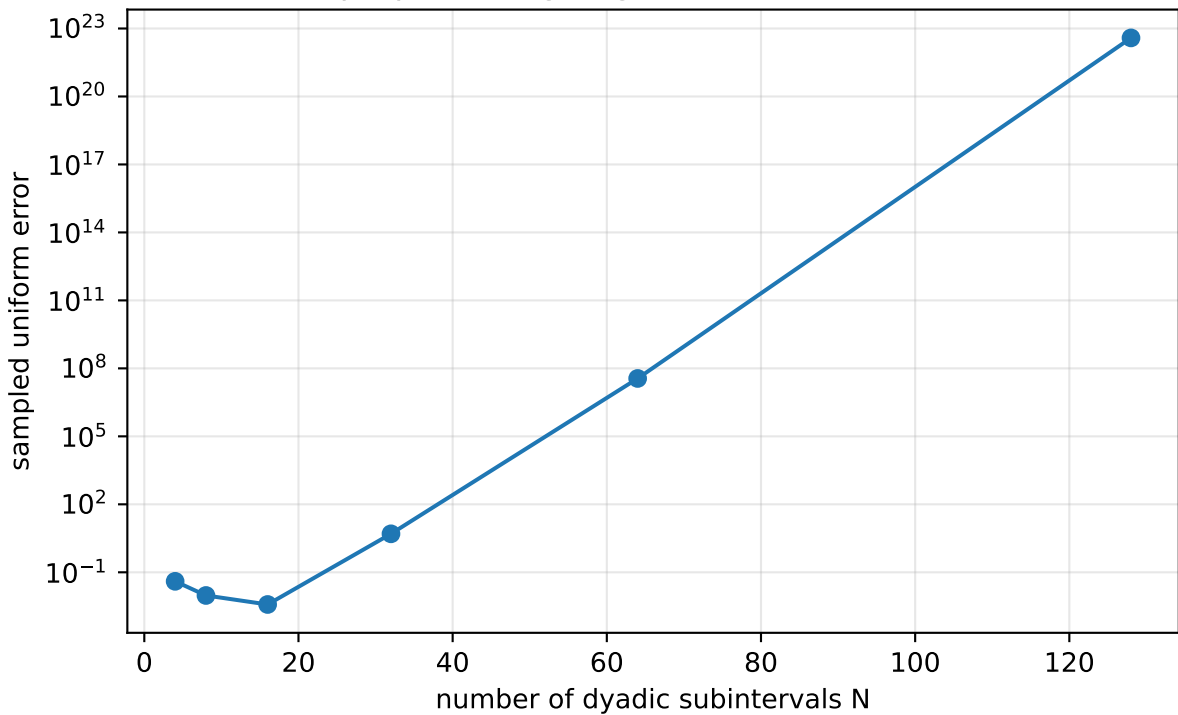
Global equispaced Lagrange error for the Fabius function
