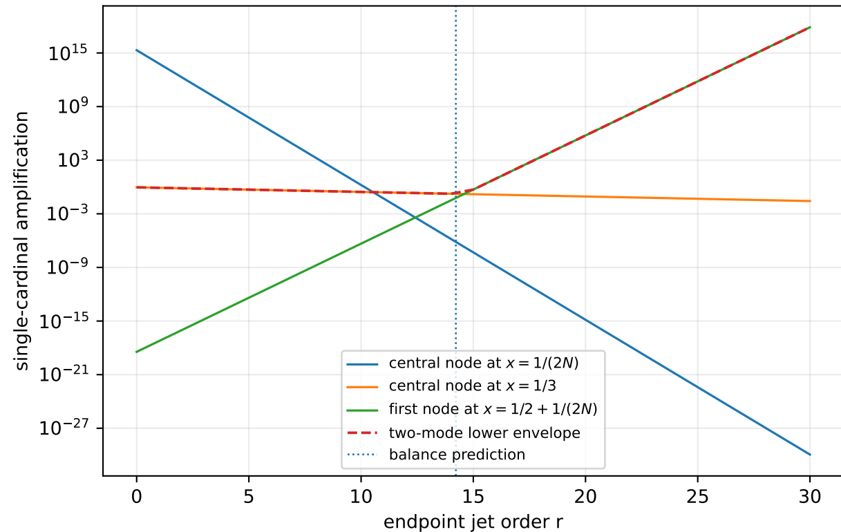
Competing instability modes for N=64
