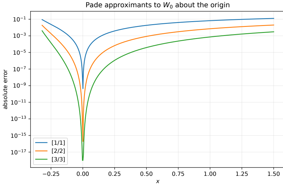
Figure 7: Absolute errors of three diagonal Pade approximants. Their main advantage over a Taylor polynomial is sensible behavior beyond the disk |x| < 1/e .
