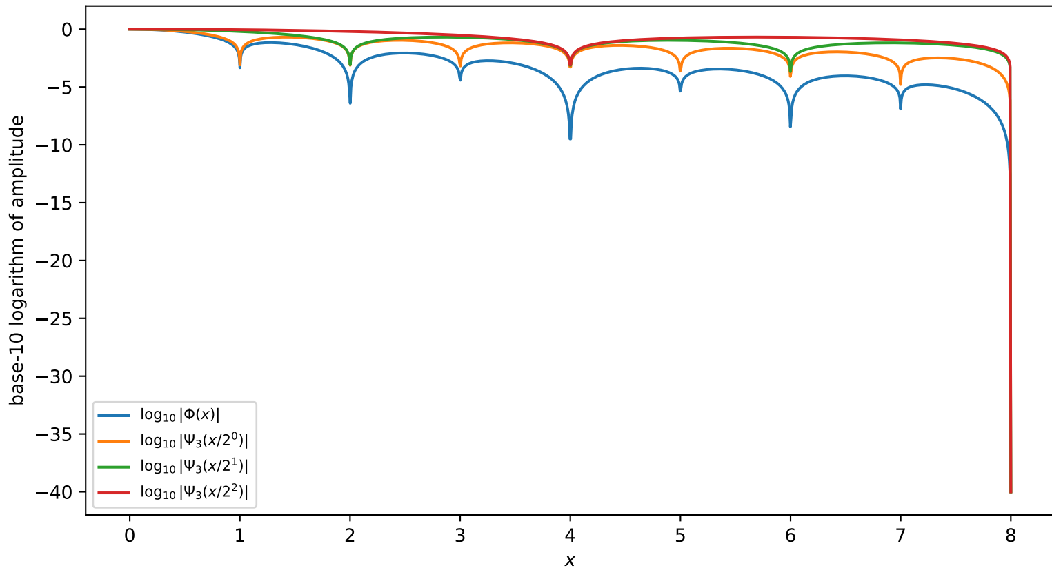
Polyphase factors of the Rvachev Fourier product
