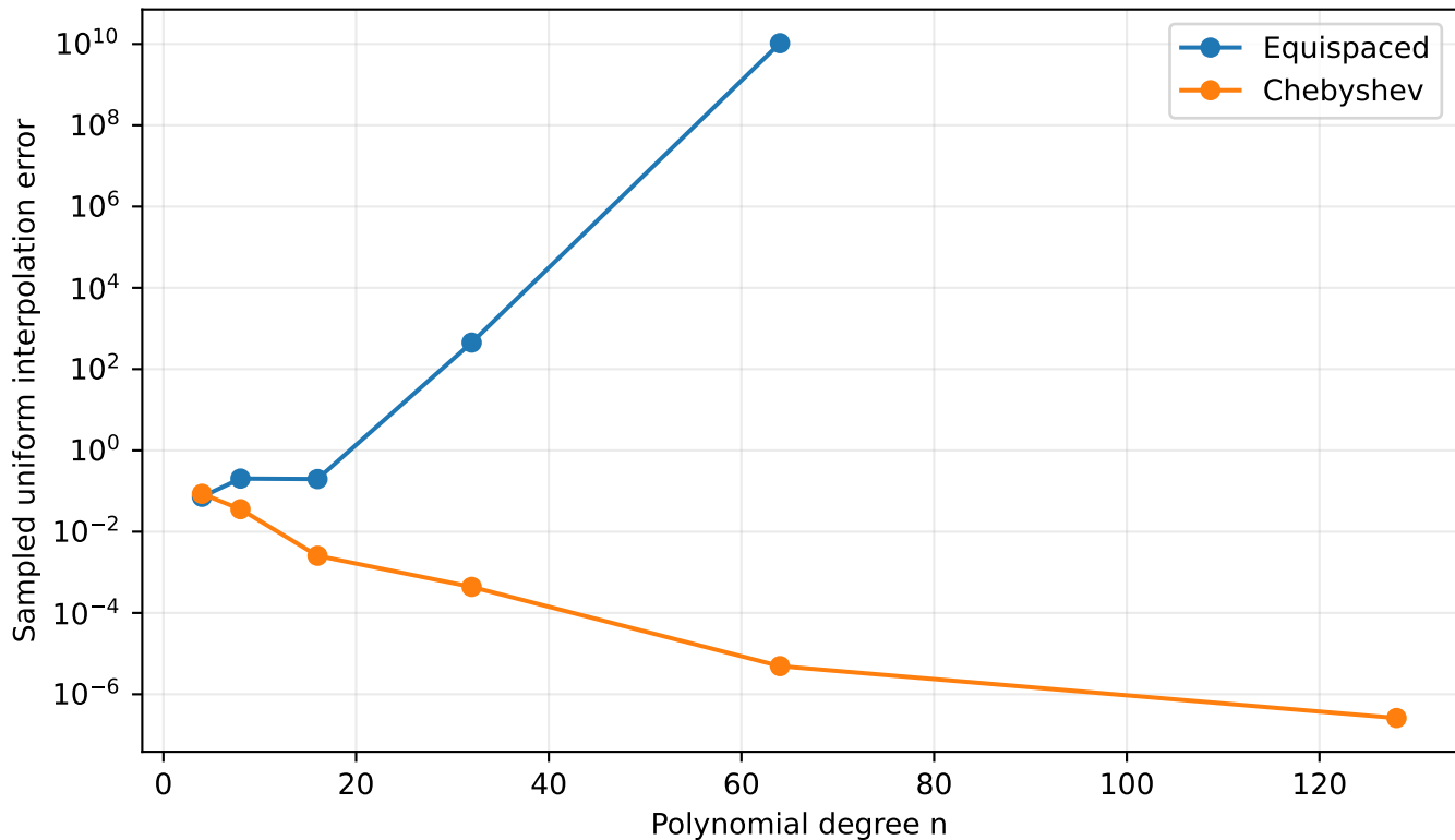
The up-shift loop inherits the Lagrange error exactly
