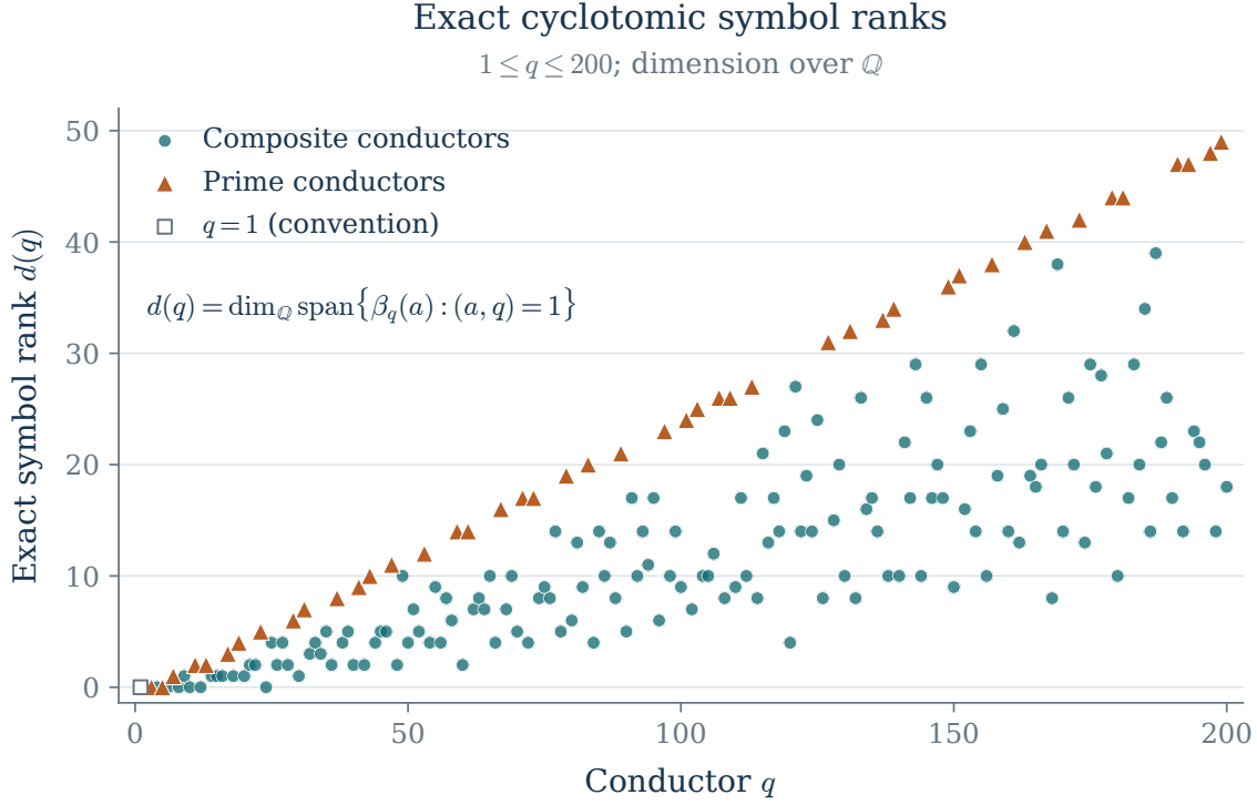
Figure 10.1: Exact ranks of the cyclotomic symbol spaces for conductors 1 \leq q \leq 200 . The plotted values come from integer residue counts and the proved rank formula. They are not numerical estimates of linear independence among evaluated periods.
