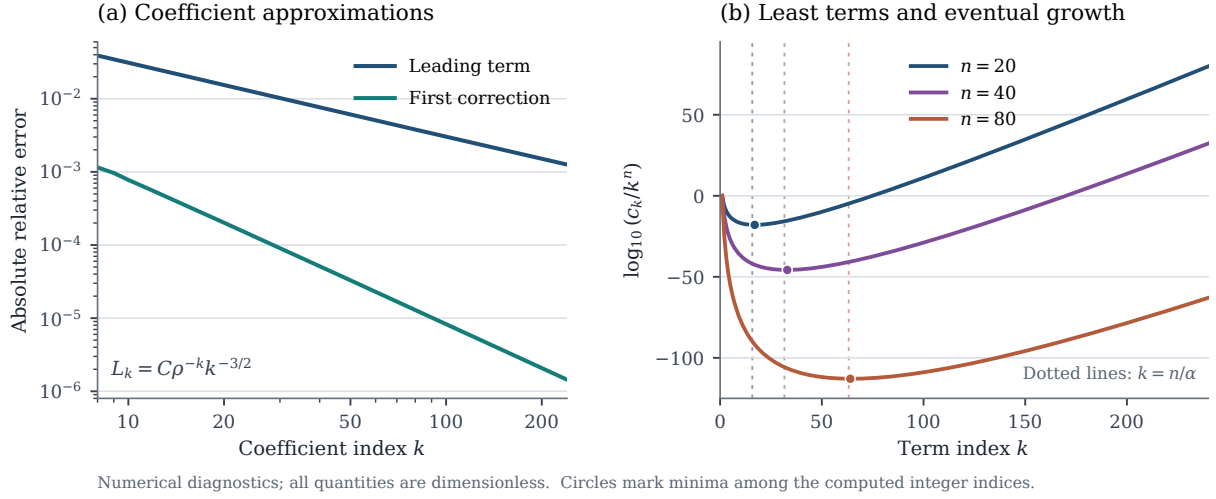
Figure 7.1: Numerical diagnostics for the proved coefficient and moment asymptotics. Left: absolute relative errors of C\rho^{-k}k^{-3/2} and C\rho^{-k}k^{-3/2}(1 + \beta_1/k) , using coefficients computed from their positive defining recurrence. Right: \log_{10}(c_k/k^n) for n = 20, 40, 80 . Dotted vertical lines mark k = n/\alpha ; circles mark the sampled minima. All plotted quantities are dimensionless. The figure illustrates the theorems and supplies no independent error certificate.
