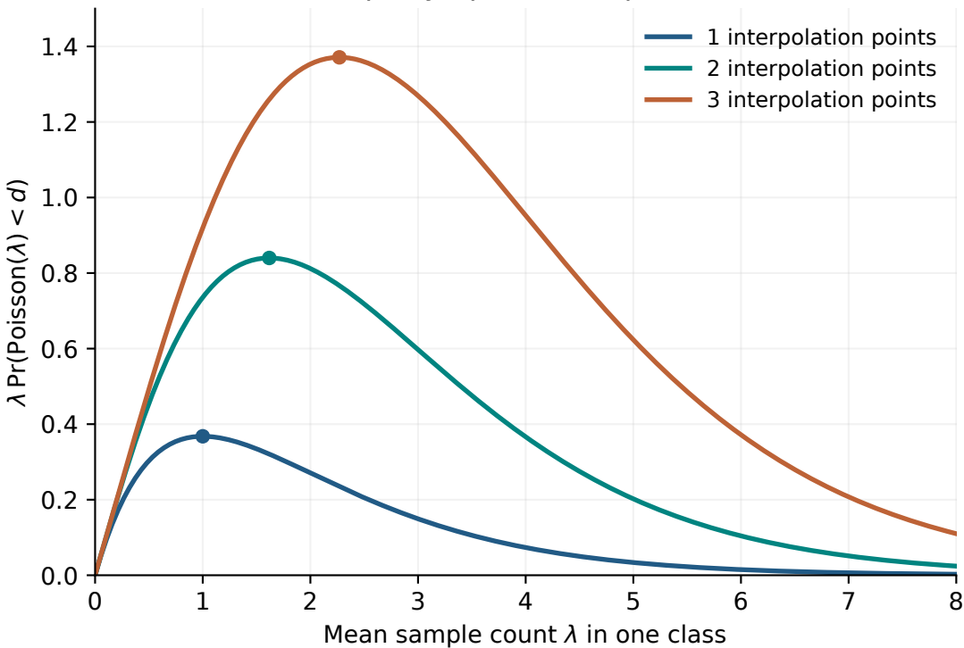
Sharp asymptotic loss per class
