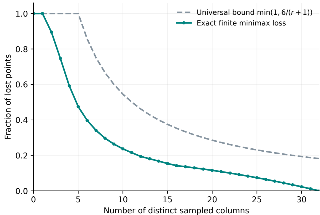
Finite example: n = 32, q = 3, d = 2
