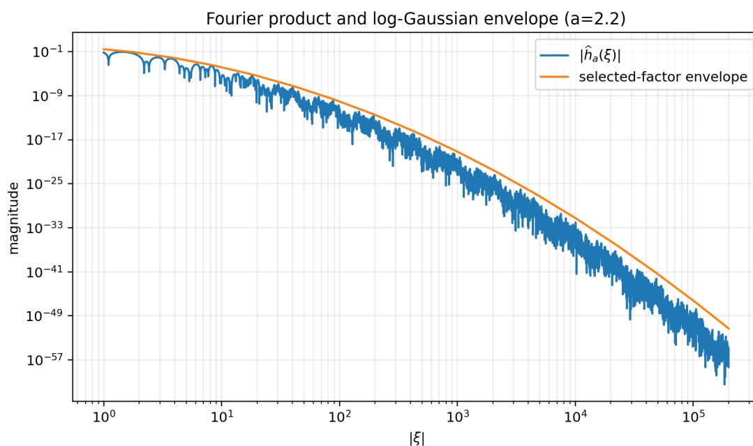
Figure 27: The Fourier product for a = 2.2 and the selected-factor bound (17.1). The oscillatory zeros sit well below the envelope, while the quadratic decay in \log |\xi| is clearly visible.
