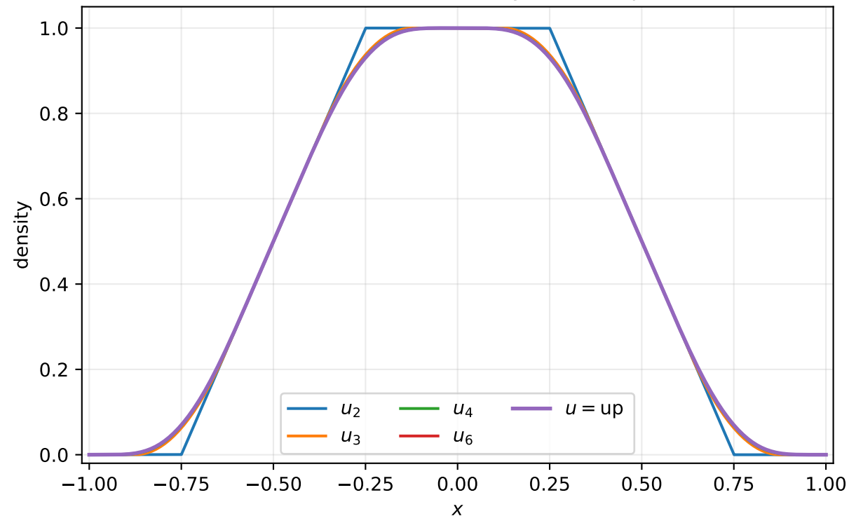
Inverse transforms of finite dyadic sinc products
