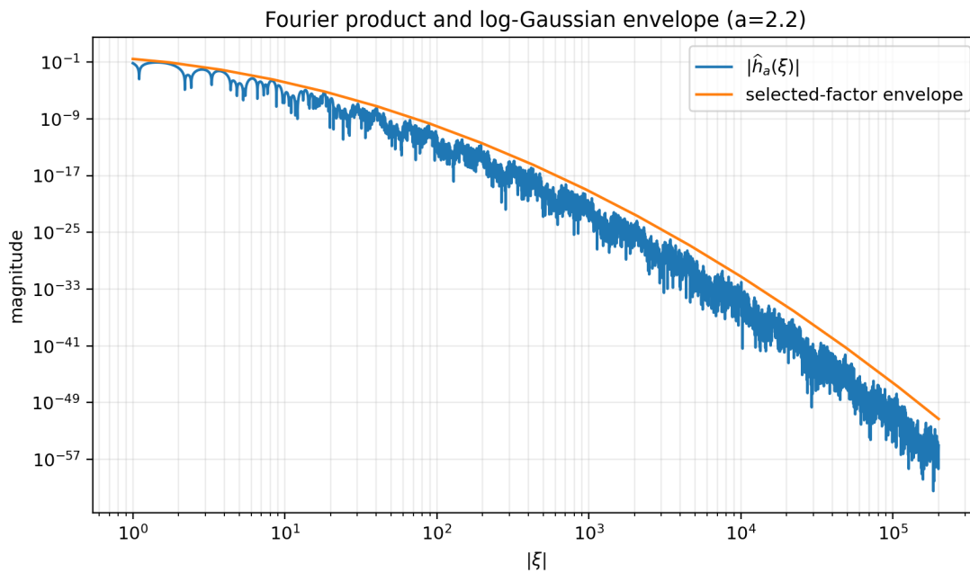
Figure 22: The Fourier product for a = 2.2 and the selected-factor bound (15.1). The oscillatory zeros sit well below the envelope, while the quadratic decay in \log |\xi| is clearly visible.
