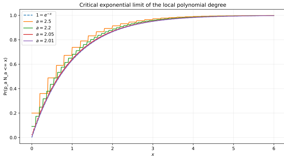
Figure 21: Distribution functions of p_a N_a approaching 1 - e^{-x} as a \downarrow 2 (theorem 13.3).
