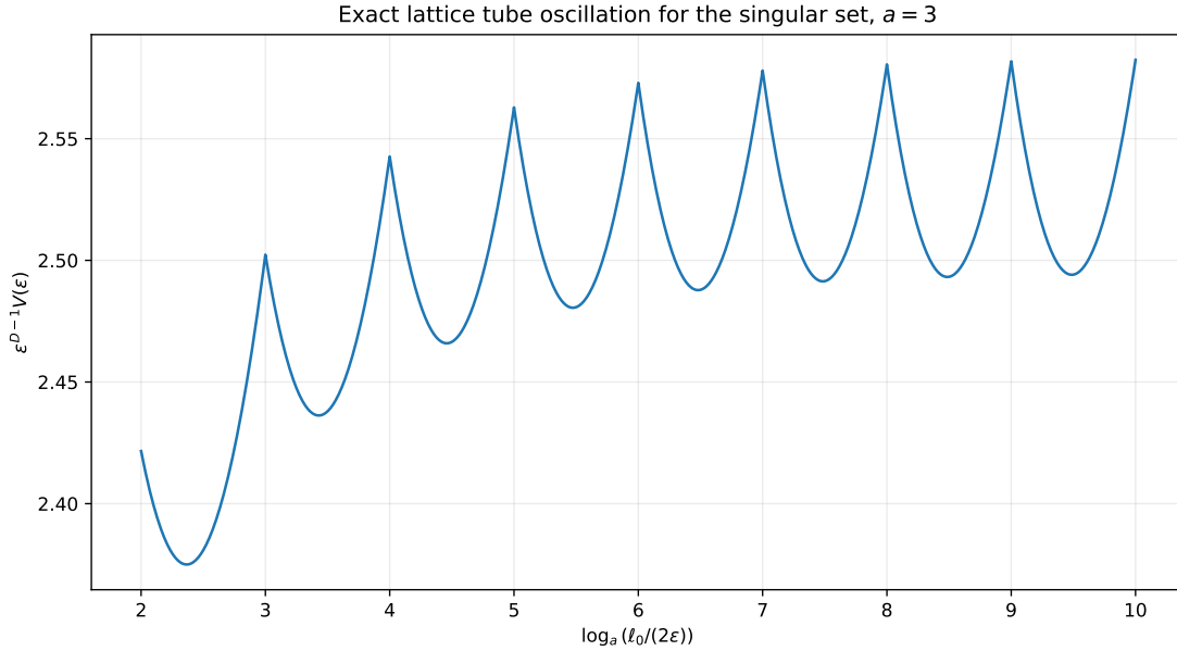
Figure 20: The exact normalized tube volume for a = 3 . The approach to a nonconstant one-periodic profile in \log_a(1/\varepsilon) verifies the lattice oscillation of theorem 13.2 .
