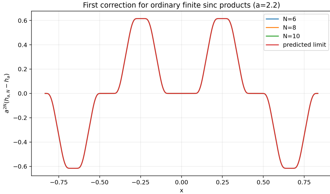
Figure 23: For a = 2.2 , the scaled errors a^{2N}(h_{a,N} - h_a) for N = 6, 8, 10 are visually indistinguishable from -h_a''/[6(a^2 - 1)] . The computation uses FFT inversion of the explicit products, not random sampling.
