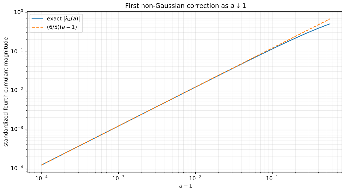
Figure 25: The exact standardized fourth cumulant (18.3) and its first asymptotic term as a \downarrow 1 .
