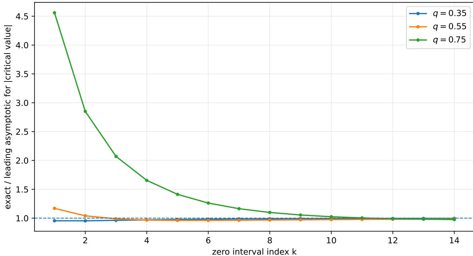
Infinite q-Pochhammer critical-value asymptotics
