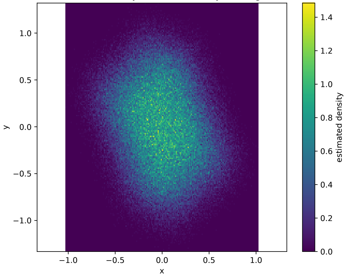
Monte Carlo density of the irrationally rotating law
