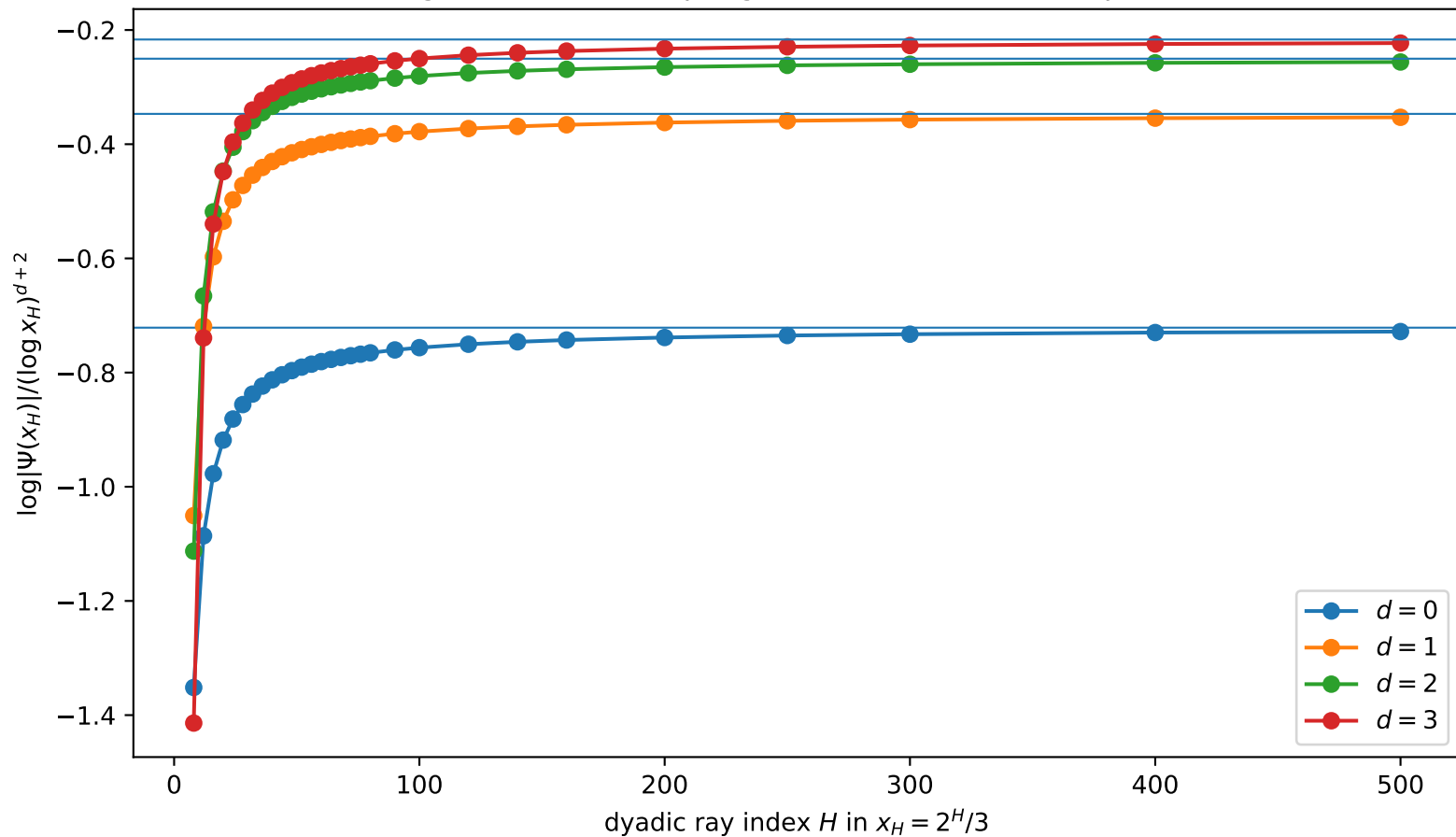
Convergence to the sharp logarithmic Fourier-envelope constant
