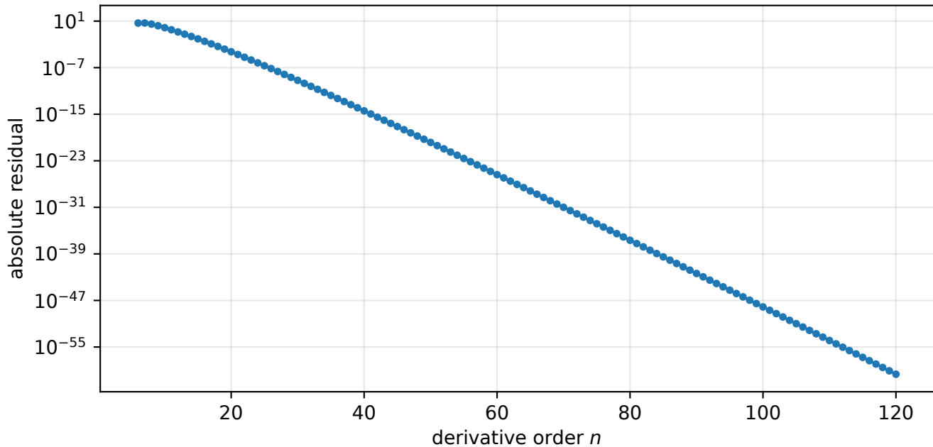
Bell-polynomial edge dominance after explicit subtraction
