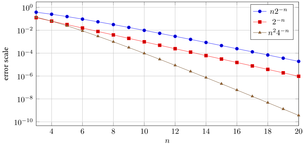
Figure 4: The three scales in (709). The deterministic center drift n2^{-n} dominates the one-cell scale 2^{-n} and the quadratic Taylor scale n^24^{-n} .
