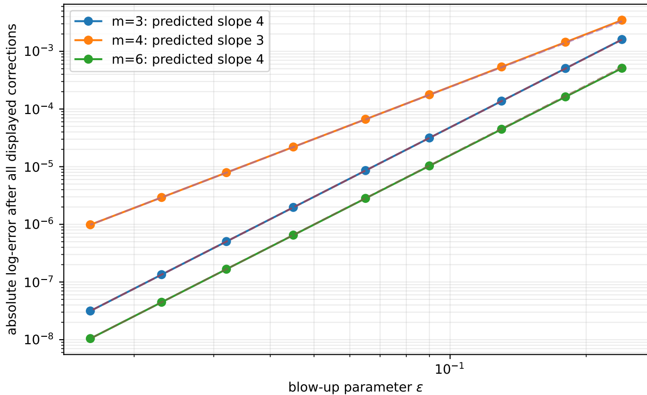
Cyclotomic blow-up: all displayed terms removed
