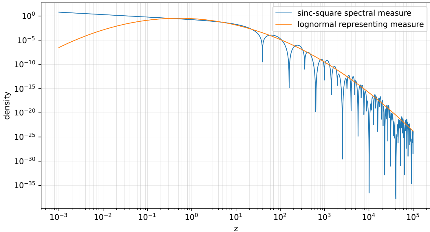
Distinct measures with moments 2^{\{n(n+1)\}}
