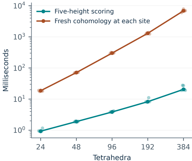
All eligible collapse scores
