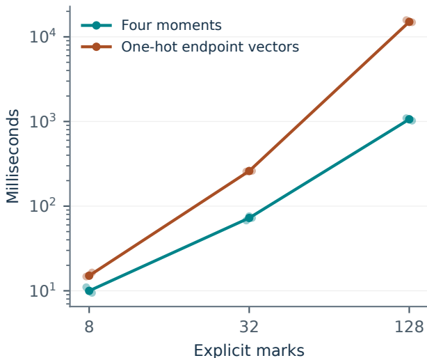
Independent marked-order replay
