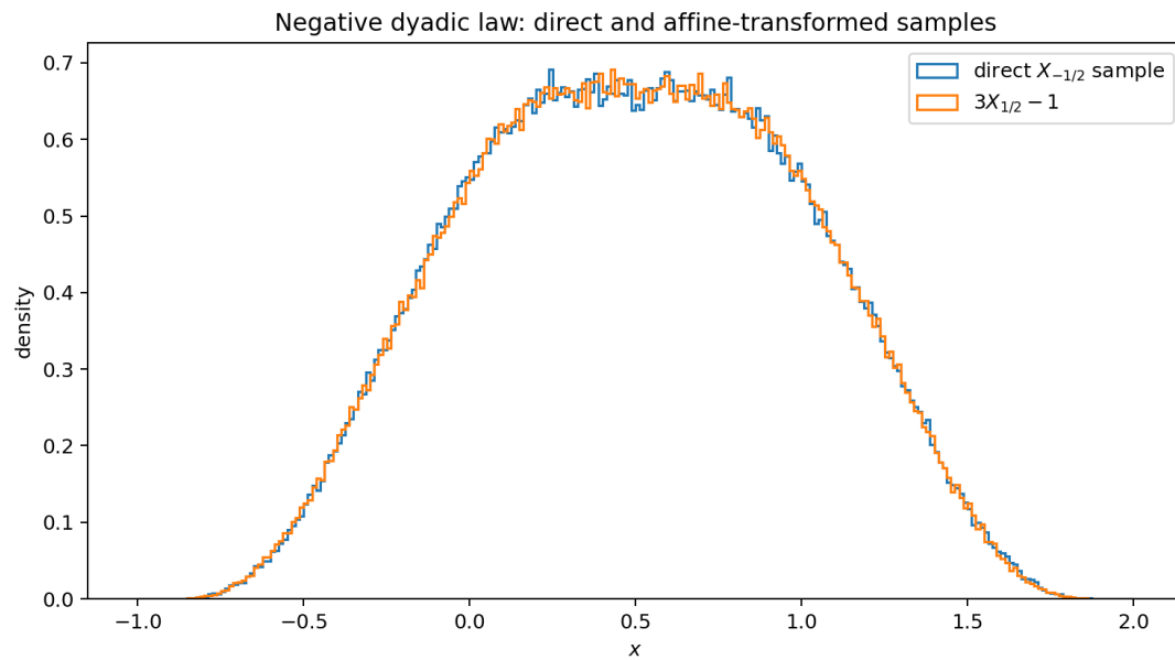
Figure 39: Independent simulations of X_{-1/2} and 3X_{1/2} - 1 . The visual agreement supplements the exact digit-reflection coupling in table 21 .
