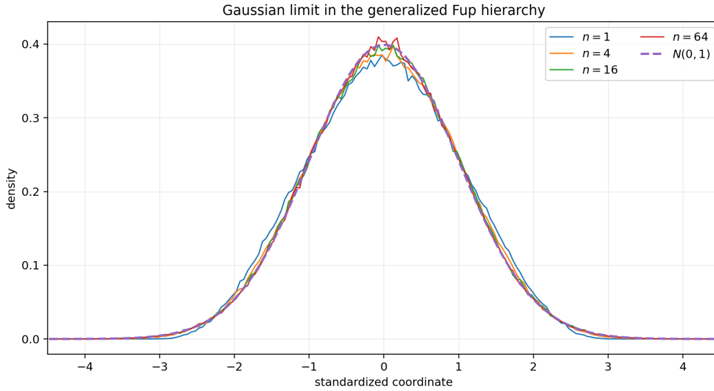
Figure 19: Standardized Fup_n densities for n = 1, 4, 16, 64 against the standard Gaussian. The exact fourth standardized cumulants are approximately -0.456, -0.214, -0.0682, -0.0183 (theorem 8.4).
