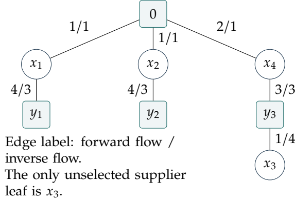
Figure 5: The common tree. Edges are drawn as undirected tree edges; transportation flow always goes from a supplier to a receiver.
