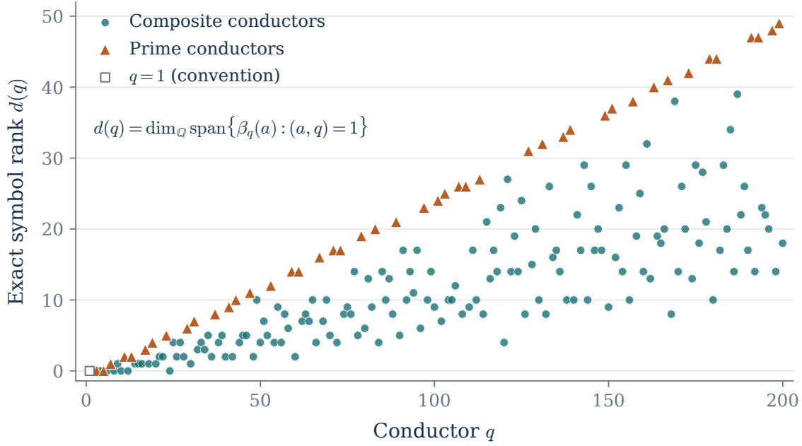
Figure 10.1: Exact ranks of the cyclotomic symbol spaces for conductors 1 \leq q \leq 200 . The plotted values come from integer residue counts and the proved rank formula. They are not numerical estimates of linear independence among evaluated periods.
