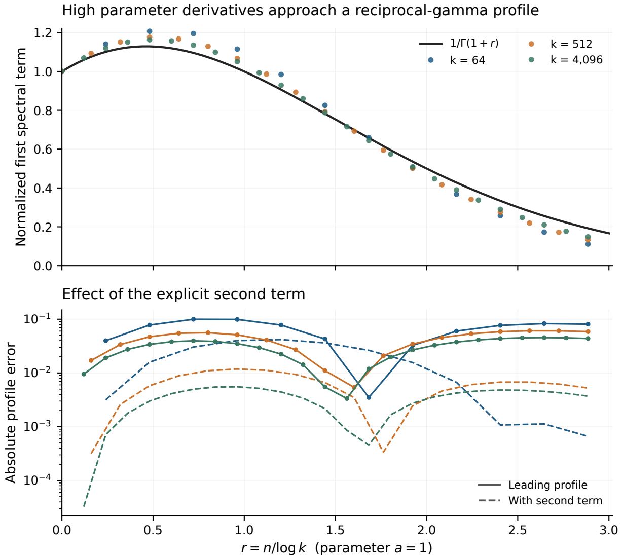
Figure 9.2: The reciprocal-gamma profile at a = 1 . The first spectral term is computed from the elementary-symmetric coefficient recurrence; its rigorously bounded spectral error is smaller than the plotted resolution. The lower panel compares its deviation from the limiting profile with its deviation after the explicit second term is included. These plotted arithmetic evaluations are floating point; the separate rational certificates do not depend on them.
