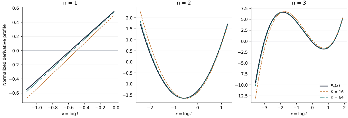
Figure 9.1: Normalized derivative profiles (1 - e^{-e^x})\mathcal{H}_{n,K}(e^x) approach P_n(x) as K = k + 1 increases. The plots illustrate n = 1, 2, 3 . Quadrature produces the curves; Theorems 9.7 and 9.11, rather than the plots, prove the zero counts and asymptotic completeness.
