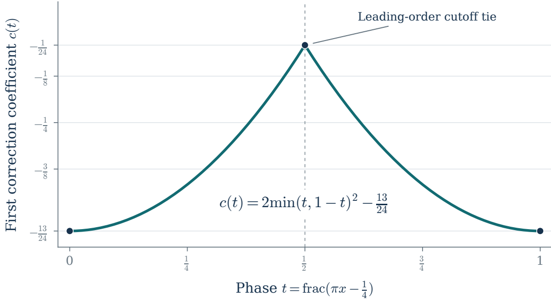
Figure 10.2: The explicit first correction in (10.57), as a function of the fractional part of \pi x - 1/4 . This plots a proved coefficient function, not fitted numerical data. The two endpoint phases represent the same point of the unit circle.
