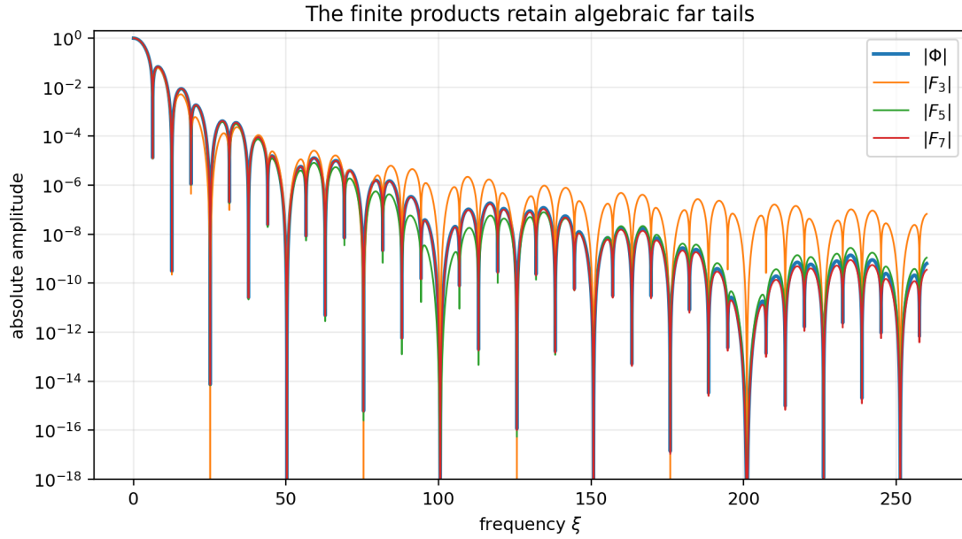
Figure 10: Absolute finite and limiting spectra on a logarithmic scale: each fixed finite product has only algebraic far-field decay ( appendix 10 ), while \Phi is rapidly decreasing; increasing n pushes the discrepancy outward to the boundary layer |t| \asymp 2^n .
