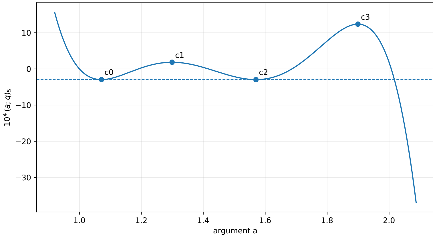
First critical-value collision for (a; q)_5 , q \approx 0.840153378
