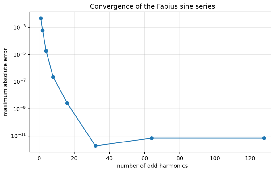
Figure 4: Maximum error of the odd-harmonic Fabius series against Fourier inversion on ten sample points.
