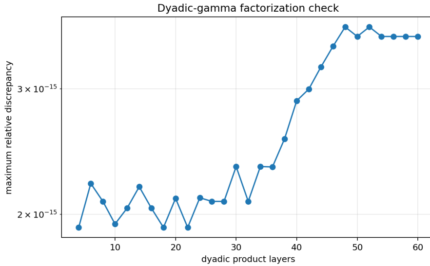
Figure 1: Finite-layer check of the dyadic-gamma reflection factorization.
