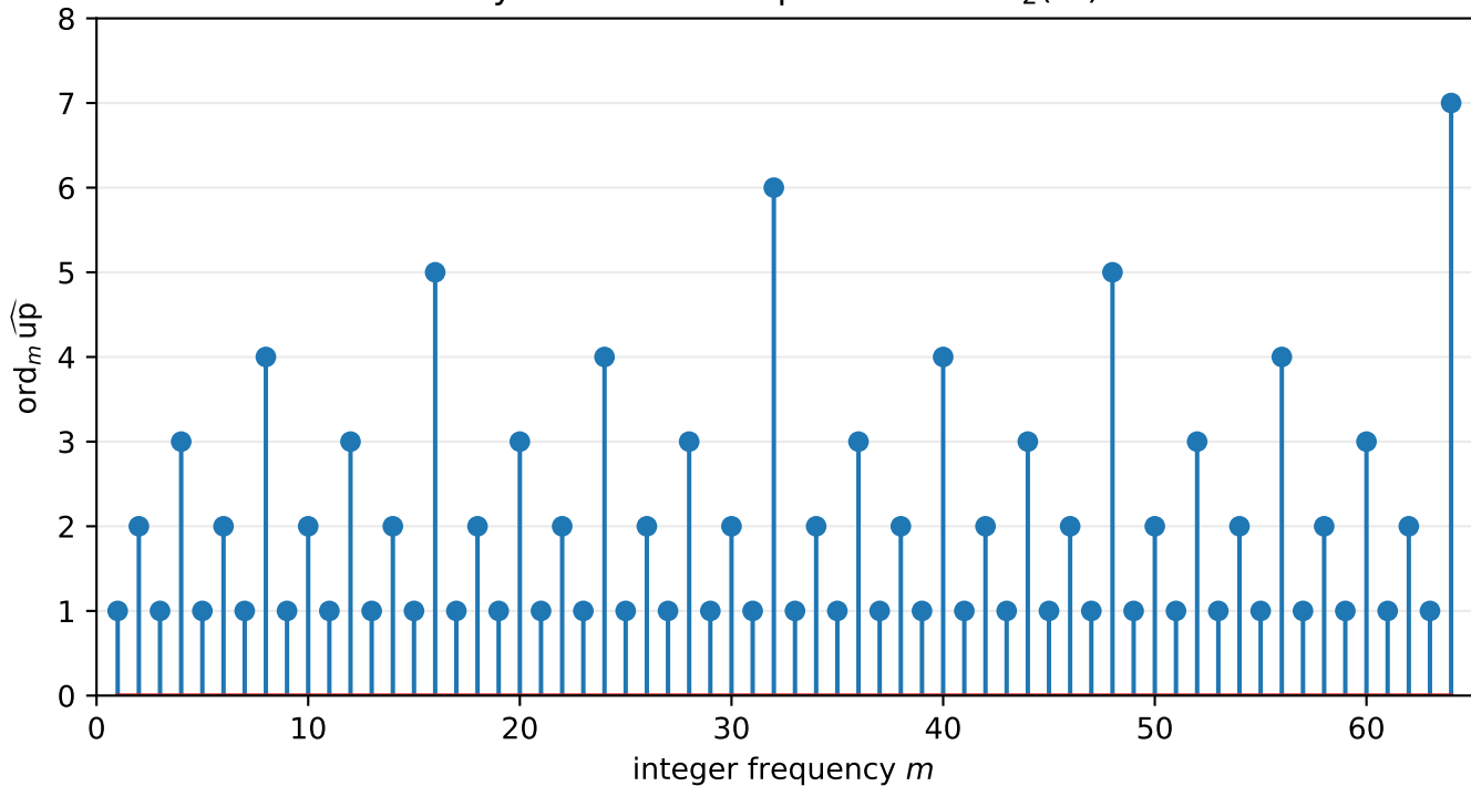
Dyadic zero multiplicities: 1 + \nu_2(m)
