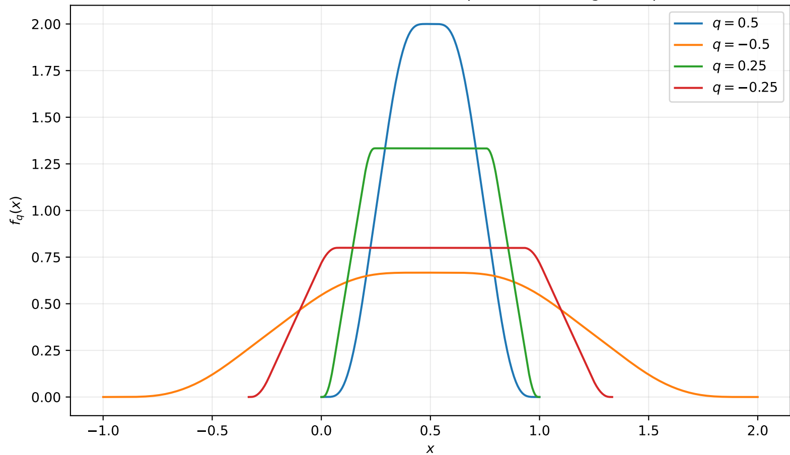
Geometric-uniform densities for positive and negative q
