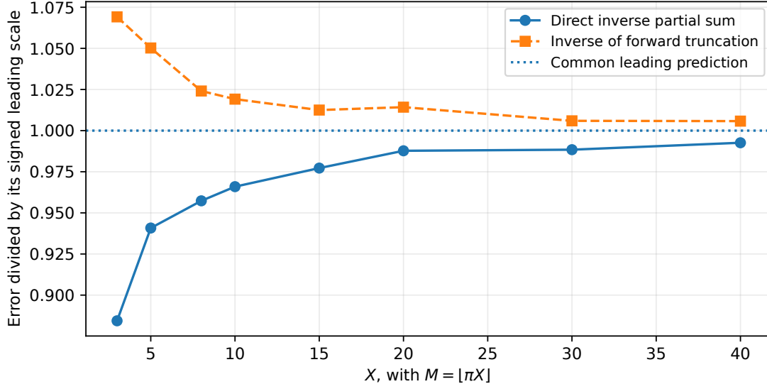
Figure 1: Recorded high-precision errors divided by (-1)^M \sqrt{X} e^{-2\pi X} , with M = \lfloor \pi X \rfloor . Both curves tend to one, but their first corrections differ. The oscillation caused by the bounded shift \sigma is retained rather than smoothed away.
