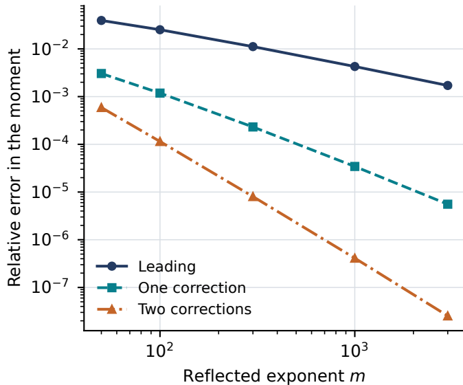
Joint log-gamma transition
