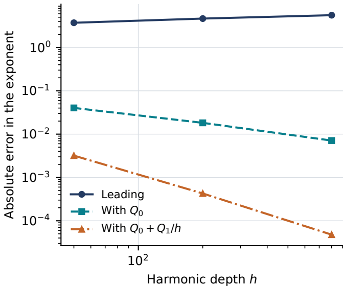
Inverse harmonic threshold
