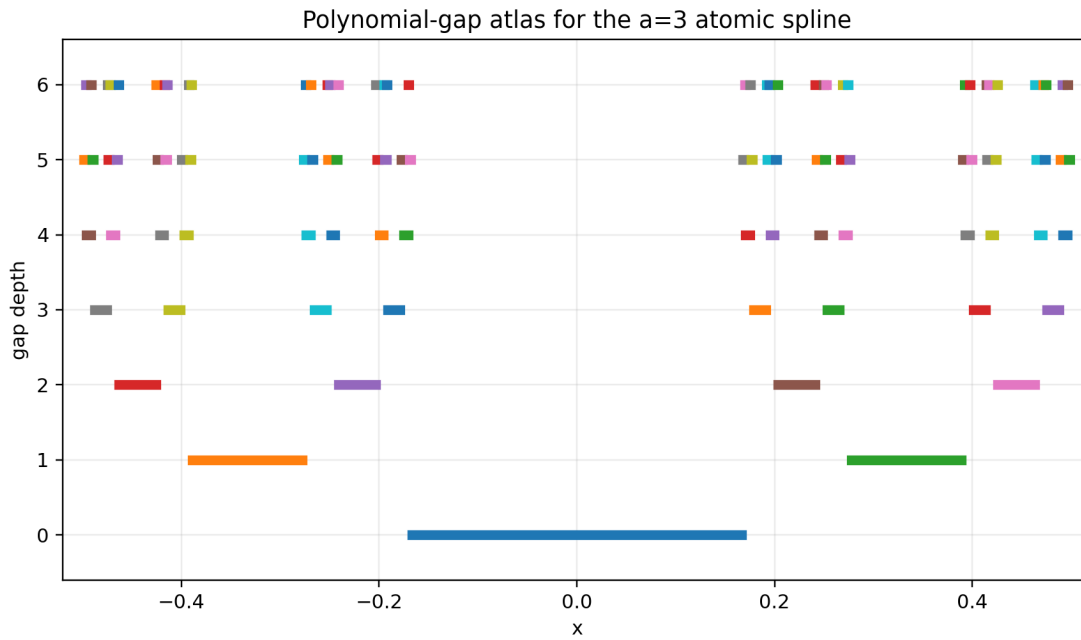
Figure 26: The first seven levels of the gap decomposition for a = 3 . The depth r gaps are the intervals on which the local polynomial degree is exactly r . Their union has full measure in the support [-1/2, 1/2] .
