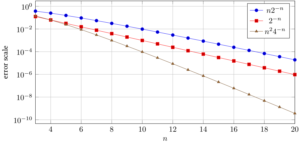
Figure 4: The three scales in (636). The deterministic center drift n2^{-n} dominates the one-cell scale 2^{-n} and the quadratic Taylor scale n^2 4^{-n} .
