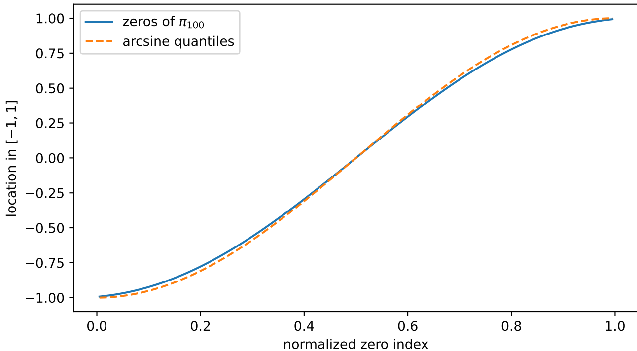
Native up-law zeros and the equilibrium distribution
