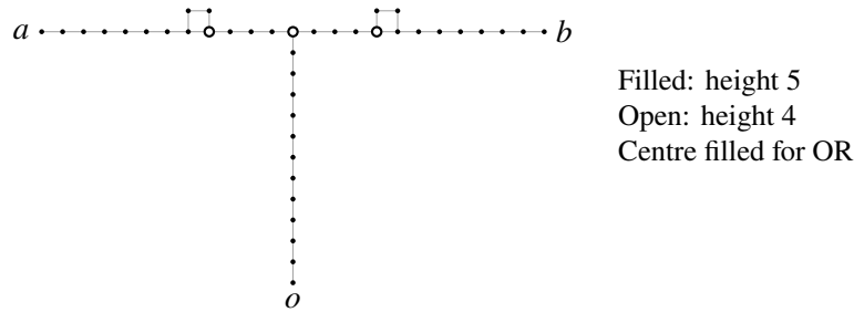
Figure 5: The literal AND template in its gate plane. The bypasses make each input logically directional although all sandpile edges are undirected.
