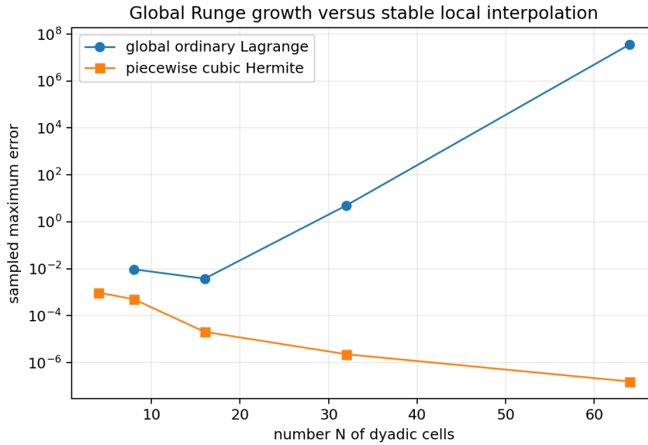
Figure 14: Global ordinary interpolation versus the cellwise cubic method on identical dyadic samples.
