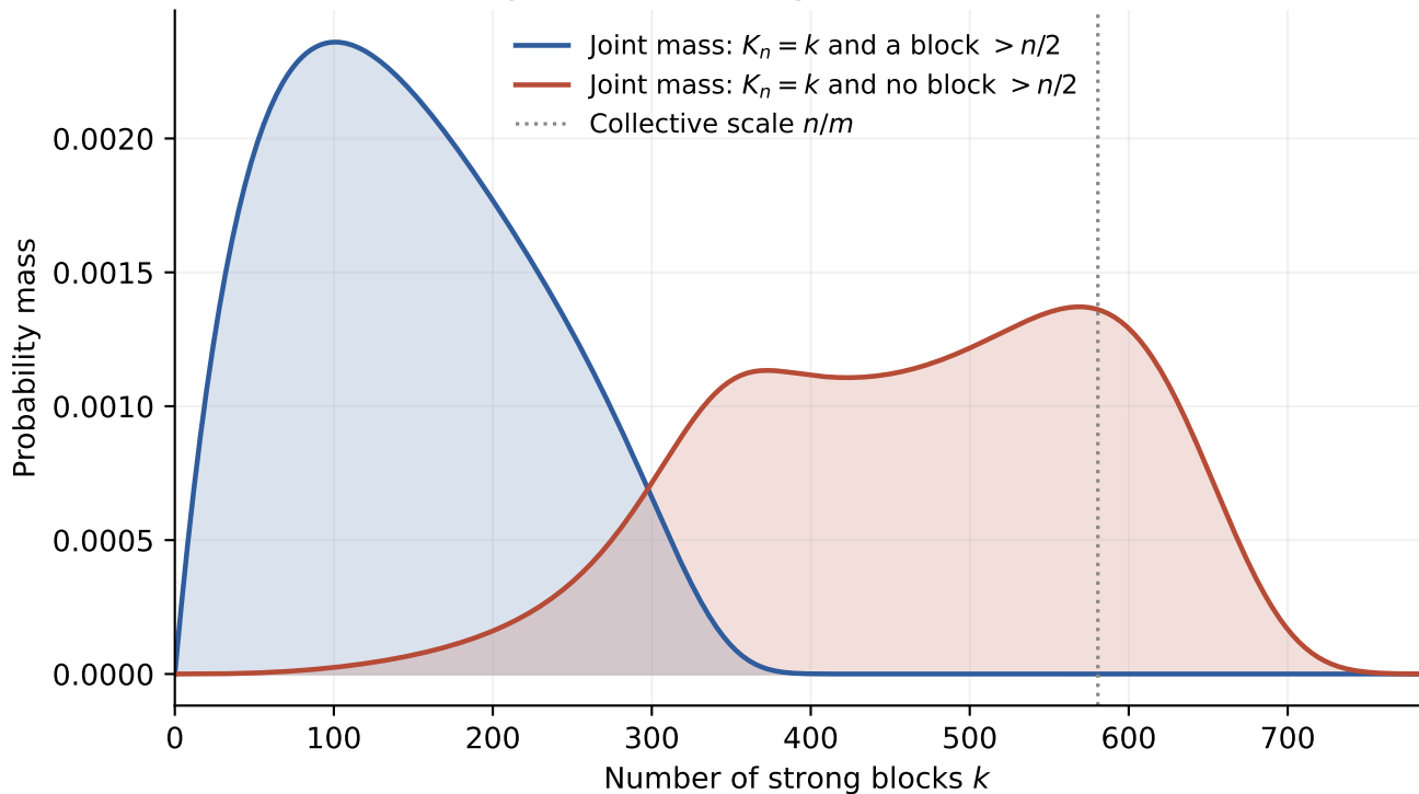
Two component-count regimes at n = 1,000 , s = 0
