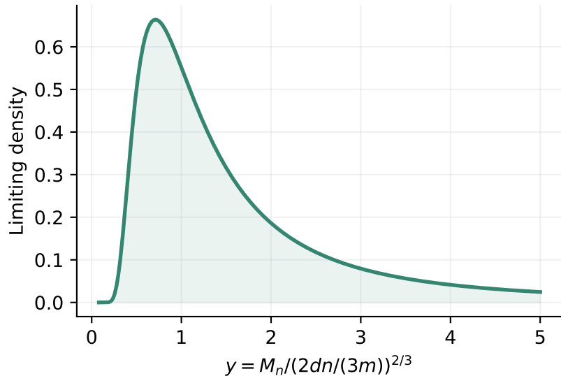
Collective phase: Fréchet maximum
