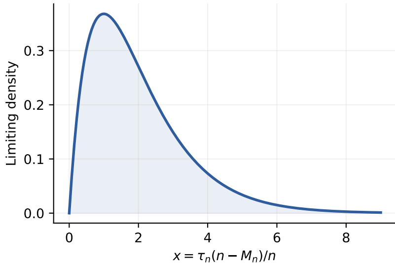
Giant phase: Gamma(2, 1) remainder
