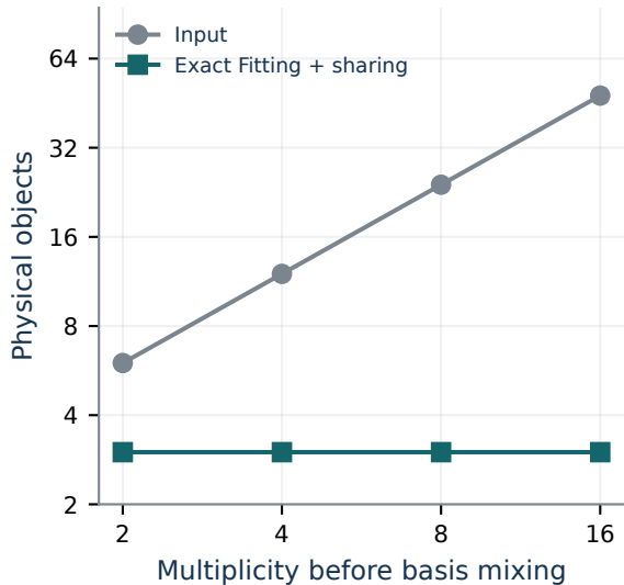
Mixed-matching constructed quivers
