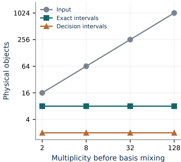
Eight-layer common-nilpotent quivers
