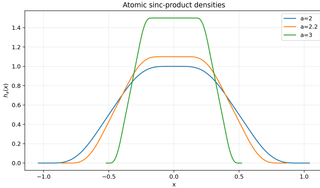
Figure 32: Profiles of h_a at the critical point a = 2 and in the separated regime. The central plateau has height a/2 and half-width (a - 2)/(a(a - 1)) for a > 2 ; it collapses to the single maximum of up at a = 2 .
