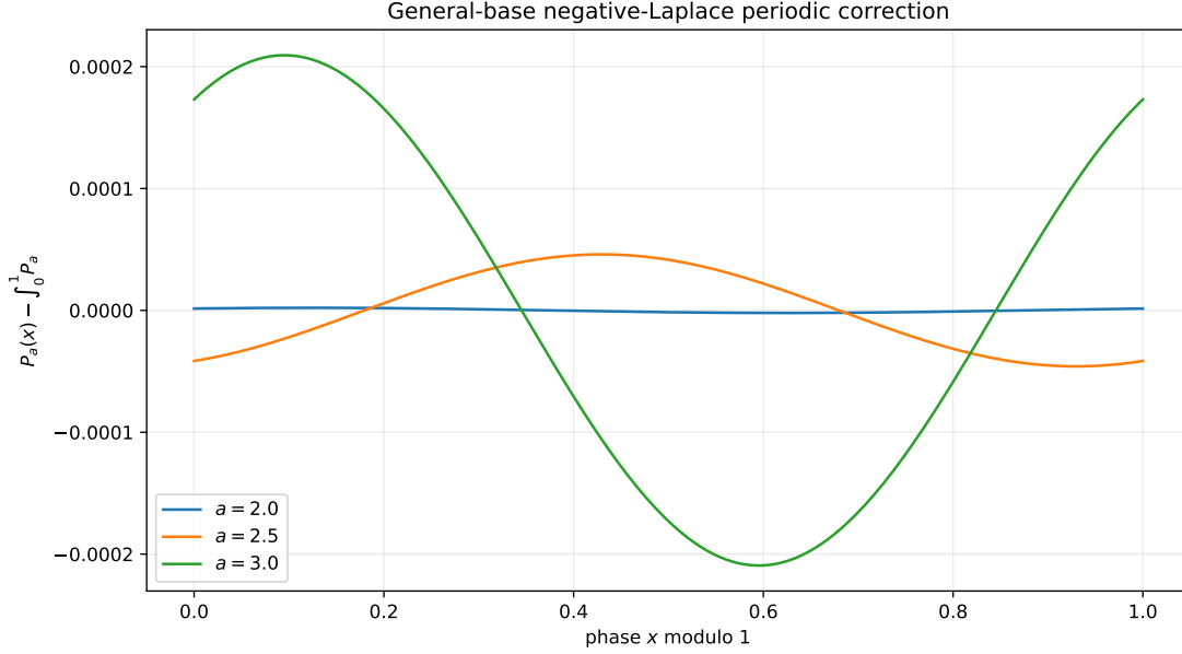
Figure 34: Centered periodic corrections \Psi_a = P_a - \bar{P}_a for several bases. The dyadic oscillation has amplitude of order 10^{-6} ; the amplitude grows substantially with the base, following the mode formula (21.17).
