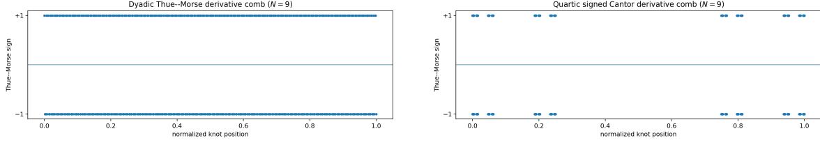
Figure 36: Signed derivative combs at level N = 9 (ordinate: Thue–Morse sign). Left, q = 1/2 : a full dyadic grid. Right, q = 1/4 : base-four digits \{0, 1\} already displaying the dimension-1/2 Cantor geometry of (12.2).
