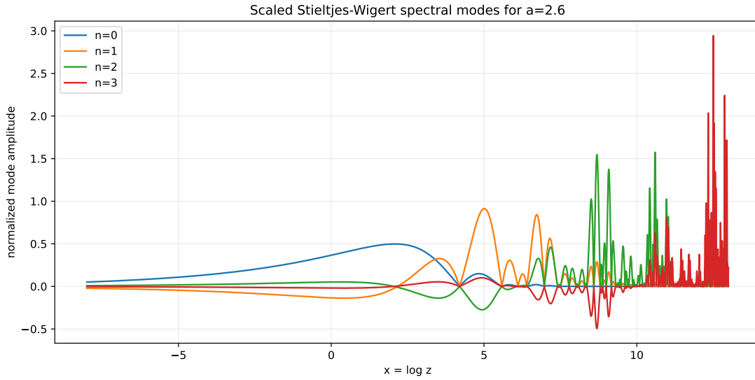
Figure 25: The first four normalized spectral modes P_{a,n}(t^2)\widehat{h}_a(t) of the differential ladder at a = 2.6 , displayed against \log(t^2) ( theorem 13.7 ). Their numerical Gram matrix is the identity to the precision recorded in the package’s orthogonal_ladder_validation_a_2_6.csv .
