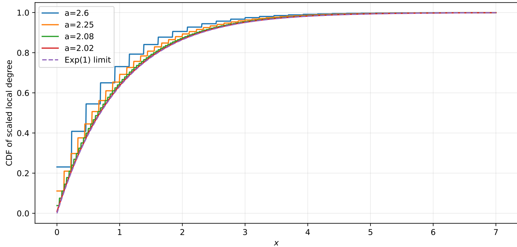
Critical local-degree limit
