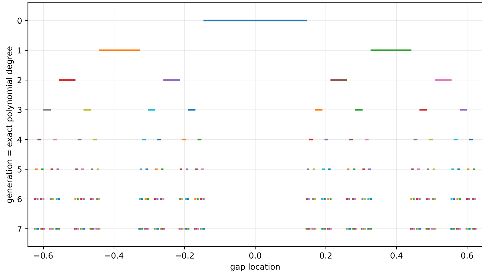
Complementary gaps of K_a for a = 2.6
