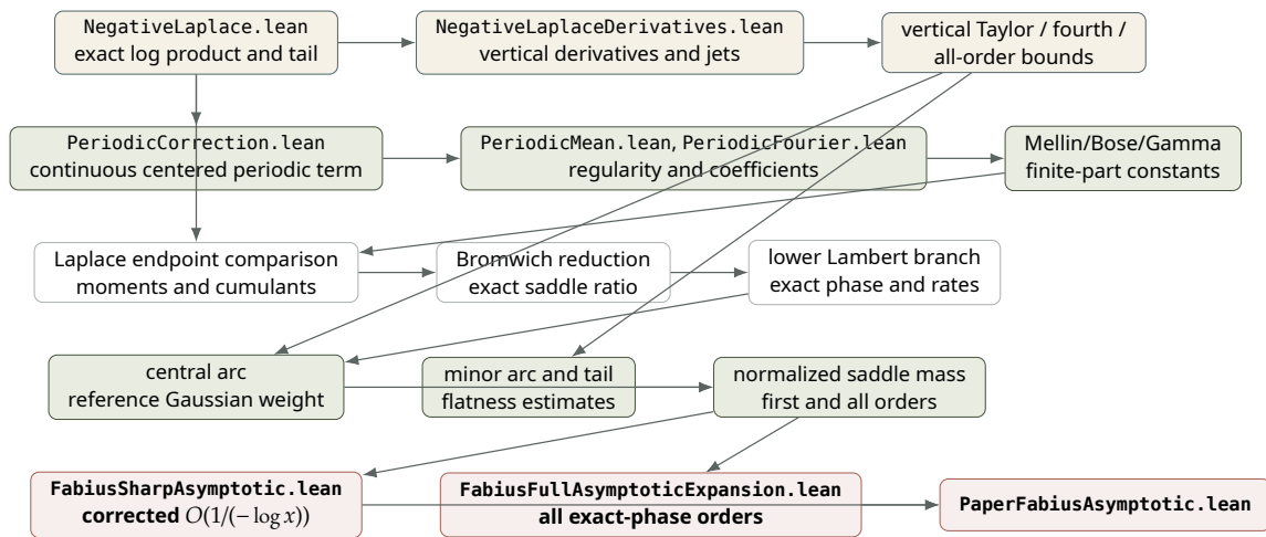
Figure 16.1: The corrected asymptotic tower. Several boxes stand for families of small modules; the direction is exact algebra \rightarrow regularization \rightarrow quantitative saddle estimates \rightarrow source-facing theorems.
