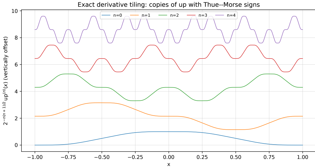
Figure 2: Normalized derivatives 2^{-T_n} up^{(n)} , vertically offset. Each row is a concatenation of copies of the original bump; their signs are the length- 2^n Thue–Morse block.
