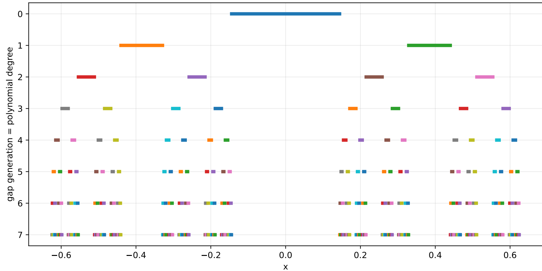
Separated gap hierarchy for a = 2.6
