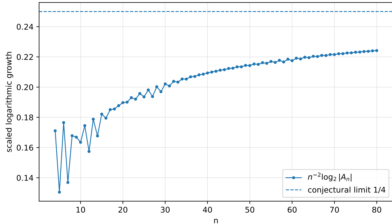
Quadratic growth of the Fabius geometric-Newton coefficients
